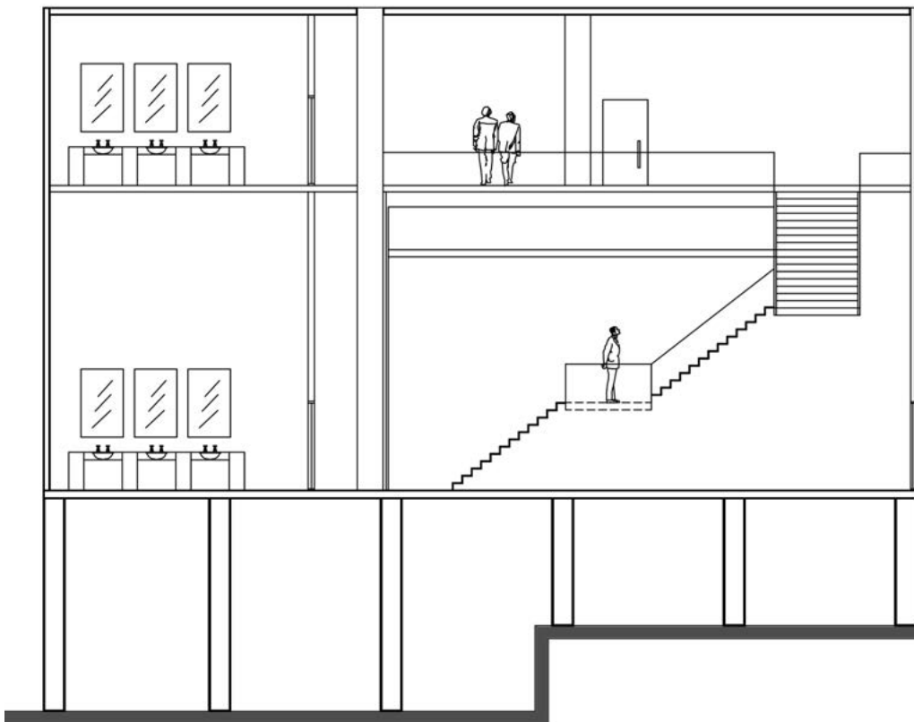
Side Section 2
