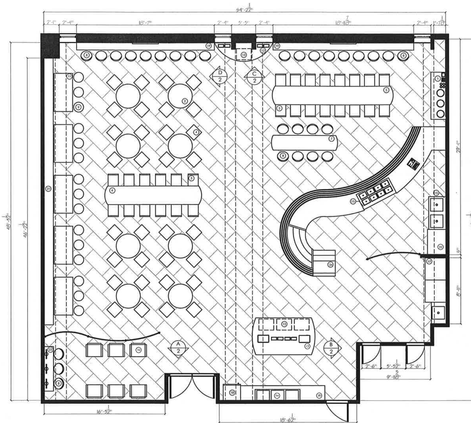
NEW PLAN of W.I.C.C. Cafeteria Scale: 1/8"=1'-0"
