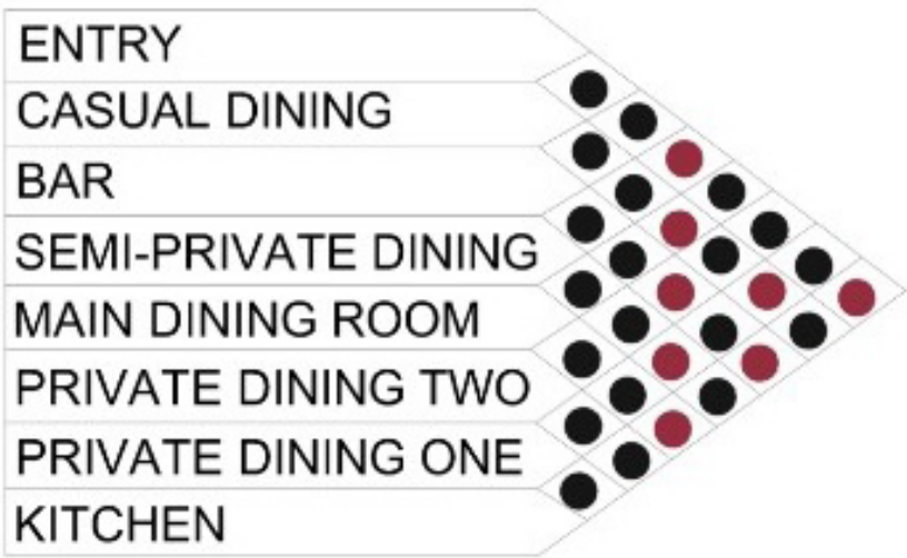
Adjacency Matrix
